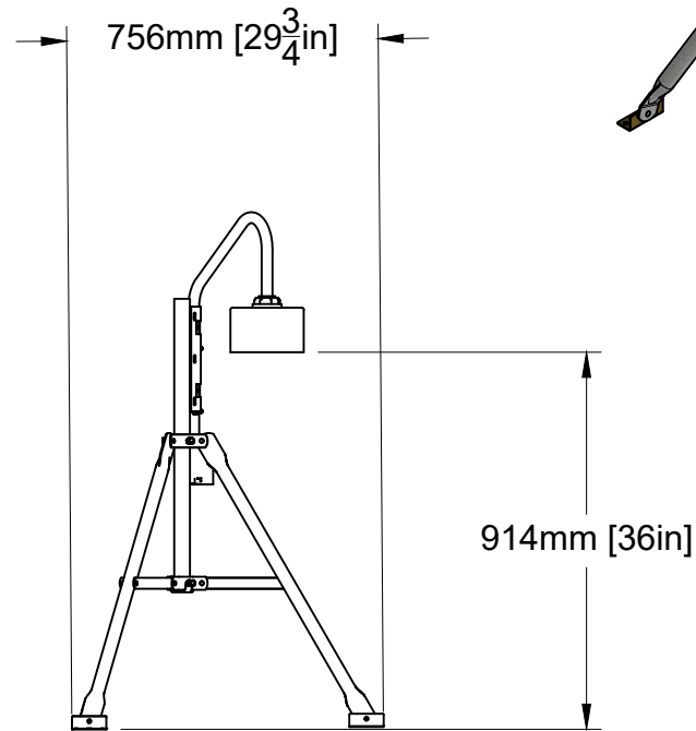
EFM-100 Sensor on TRI-3 Tripod
